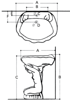
Venus Lavabo Wash-basin - Lavabo Lavabo - Waschbecken
